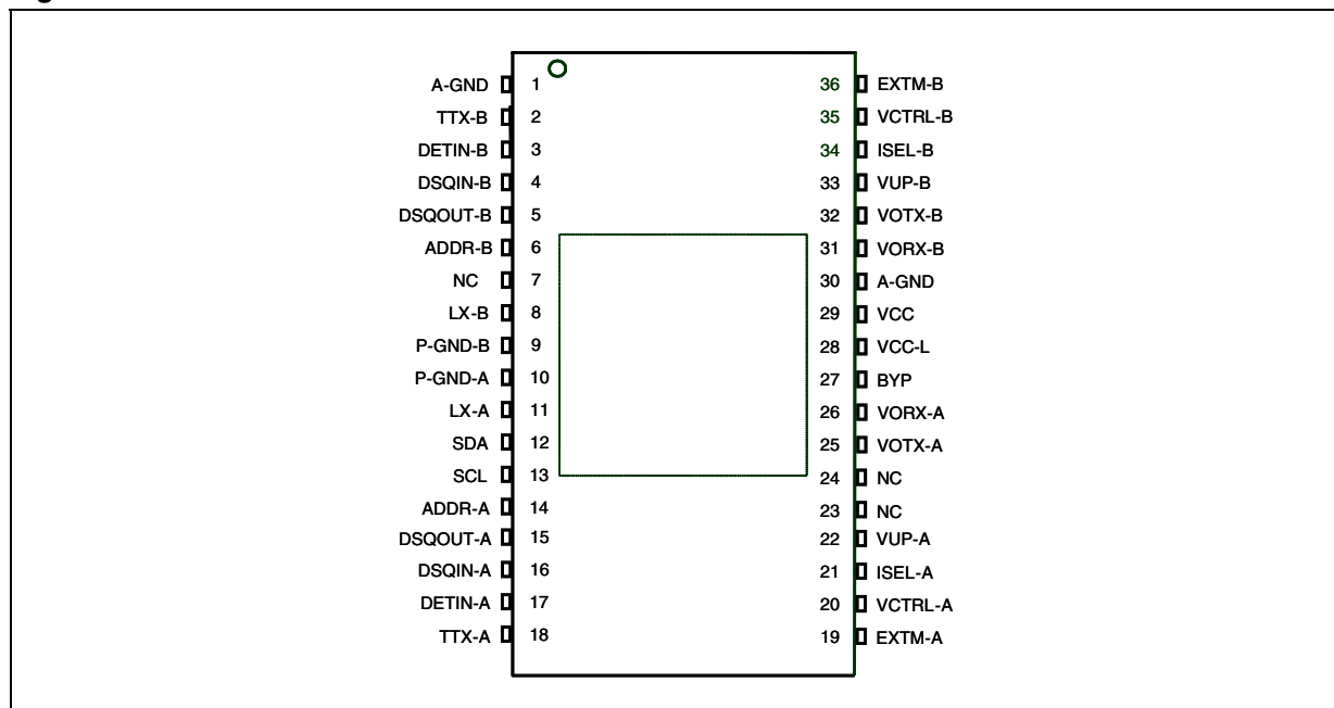
Figure 3. Pin connections
